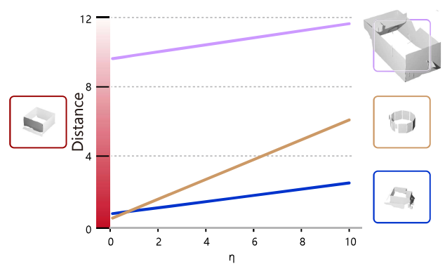
Fig. 16. Impact of the shape-scale balance weight \eta on segment similarity: Increasing \eta shifts the metric emphasis from scale to shape similarity.
