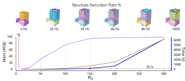
Fig. 15. Relationship between n_s and computational cost, benchmarked at n_s = 300 for SDR calculations. Increasing n_s improves detection of fine structures but incurs a non-linear rise in computational costs.
