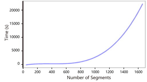
Fig. 21. The relationship between the calculation time of the co-analysis stage and the number of segments analyzed simultaneously.
